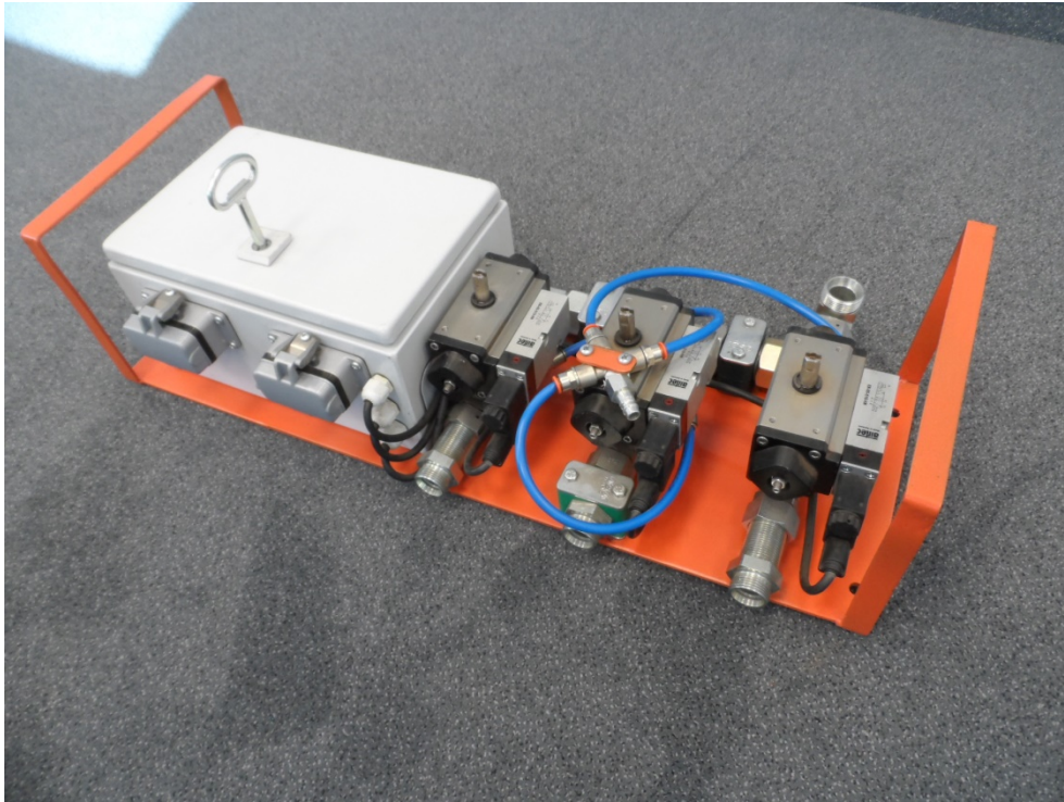
Dimensions (L/H/W) 750/250/190 mm - Weight: 25 kg
